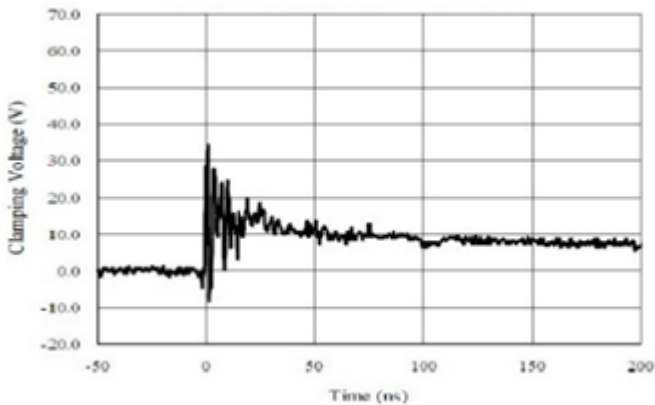
FIGURE 5 ESD Clamping (+8 kV Contact Per IEC 61000-4-2)
