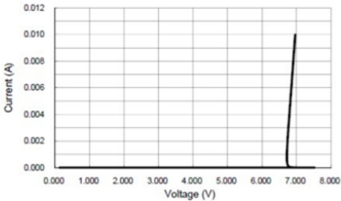
FIGURE 3 Voltage Sweeping
