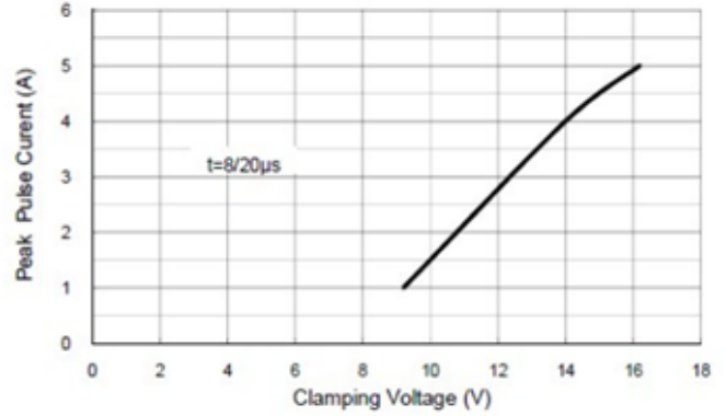
FIGURE 2 Clamping Voltage VS. Peak Pulse Current
