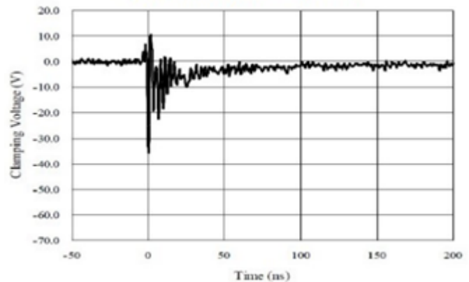
FIGURE 6 ESD Clamping (-8 kV Contact Per IEC 61000-4-2)
