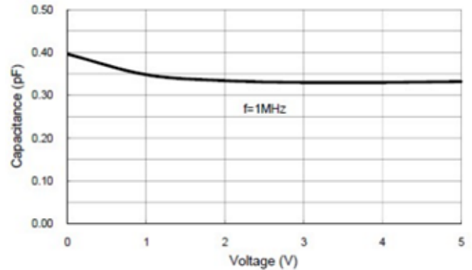
FIGURE 4 Voltage VS. Capacitance
